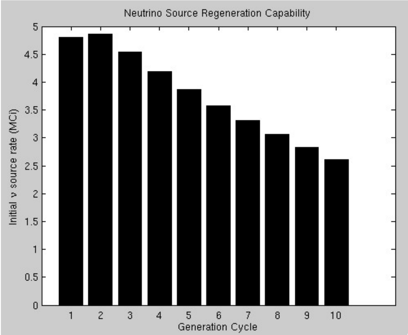
Recharging ^{51}\text{Cr} source (37.6MCi equivalent), M. Pyle
