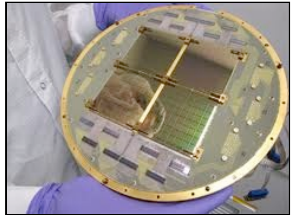
SCUBA II Detector (10,000 pixels, each extremely small)
